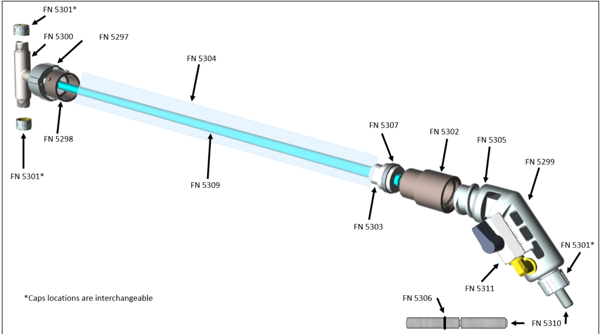
Figure 4: Component Diagram
