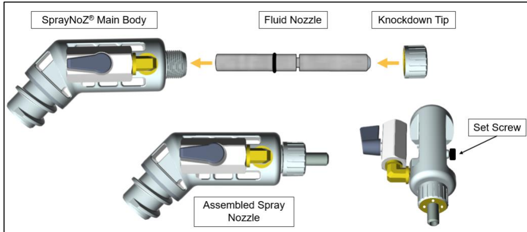
Figure 3: Main Body setup
